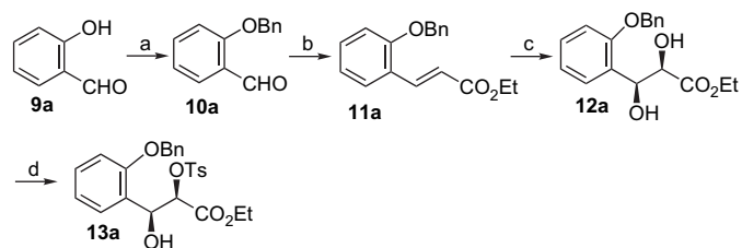
Scheme 1. Reagents and conditions: (a) BnBr, anhyd K_2CO_3 , dry acetone, reflux, 4 h, 85%; (b) Ph_3P=CHCO_2Et , dry CH_2Cl_2 , rt, 2 h, 78%; (c) AD-mix- \alpha , t -BuOH/ H_2O (1:1), 0 °C, 28 h, 92%; (d) TsCl, dry Et_3N , dry CH_2Cl_2 , 0 °C, 72 h, 87%.
