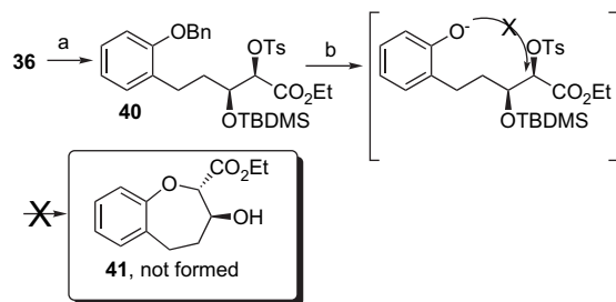
Scheme 9. Reagents and conditions: (a) TBDMS-OTf, 2,6-lutidine, 0 °C–rt, 8 h, 85%; (b) (i) H 2 , 10% Pd/C, ethyl acetate; (ii) anhyd K 2 CO 3 , dry acetone, reflux, 15 h.
