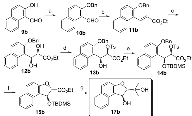
Scheme 3. Reagents and conditions: (a) BnBr, anhyd K_2CO_3 , dry acetone, reflux, 4 h, 83%; (b) Ph_3P=CHCO_2Et , dry CH_2Cl_2 , rt, 2 h, 80%. (c) AD-mix- \alpha , t -BuOH/ H_2O (1:1), 0 °C, 28 h, 93%; (d) TsCl, dry Et_3N , dry CH_2Cl_2 , 0 °C, 72 h, 94%; (e) TBDMS-OTf, 2,6-lutidine, 0 °C–rt, 6 h, 88%; (f) (i) H_2 , 10% Pd/C, EtOAc, 4 h; (ii) anhyd K_2CO_3 , dry acetone, 6 h, 72% (based on two steps); (g) (i) MeMgI, dry ether, reflux, 4 h; (ii) TBAF, dry THF, 0 °C, 5 h, 74% for two steps.
