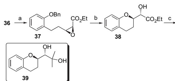
Scheme 8. Reagents and conditions: (a) anhyd K 2 CO 3 , ethanol, 8 h, 78%; (b) (i) H 2 , 10% Pd/C, ethyl acetate, 2 h; (ii) anhyd K 2 CO 3 , dry acetone, 6 h, (68%, for two steps); (c) MeMgI, dry ether, reflux, 4 h, 83%.
