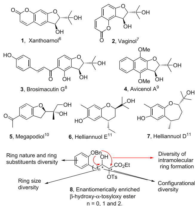
Figure 1. Bioactive natural products (1–7) containing benzo-annulated oxaheterocycles and the synthetic versatility of \beta -hydroxy- \alpha -tosyloxy esters (8) in our synthetic strategy.
