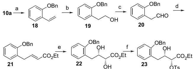
Scheme 4. Reagents and conditions: (a) methyltriphenylphosphonium iodide, t -BuOK, dry THF, 0 °C–rt, 2 h, 80%; (b) (i) 9-BBN, dry THF, 0 °C–rt, overnight; (ii) NaOH/H 2 O 2 , reflux, 2 h, 96%; (c) PCC, dry CH 2 Cl 2 , 2 h, 0 °C–rt, 76%; (d) Ph 3 P=CHCO 2 Et, dry CH 2 Cl 2 , rt, overnight, 75%; (e) AD-mix- \alpha , t -BuOH/H 2 O (1:1), 0 °C, 40 h, 89%; (f) TsCl, dry Et 3 N, dry CH 2 Cl 2 , 0 °C, 72 h, 85%.
