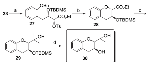
Scheme 6. Reagents and conditions: (a) TBDMS-OTf, 2,6-lutidine, 0 °C–rt, 6 h, 89%; (b) (i) H 2 , 10% Pd/C, EtOAc, 4 h; (ii) anhyd K 2 CO 3 , dry acetone, 8 h (70%, based on two steps); (c) MeMgI, dry ether, reflux, 4 h, 91%; (d) TBAF, dry THF, 0 °C, 5 h, 87%.
