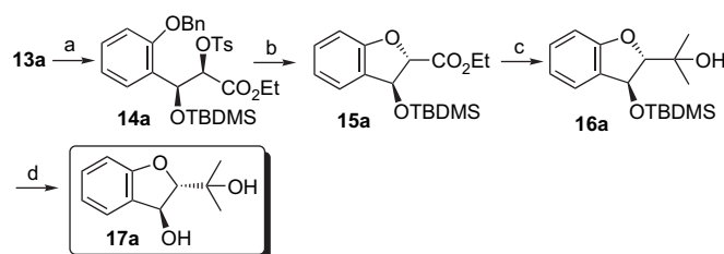
Scheme 2. Reagents and conditions: (a) TBDMS-OTf, 2,6-lutidine, 0 °C–rt, 6 h, 85%; (b) (i) H_2 , 10% Pd/C, EtOAc, 4 h; (ii) anhyd K_2CO_3 , dry acetone, 6 h, 69% (based on two steps); (c) MeMgI, dry ether, reflux, 4 h, 77%; (d) TBAF, dry THF, 0 °C, 5 h, 91%.
