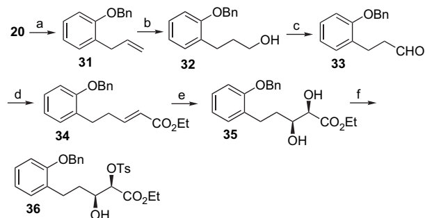
Scheme 7. Reagents and conditions: (a) methyltriphenylphosphonium iodide, t -BuOK, dry THF, 0 °C–rt, 2 h, 88%; (b) (i) 9-BBN, dry THF, 0 °C–rt, overnight; (ii) NaOH/H 2 O 2 , reflux, 2 h, 96%; (c) PCC, dry DCM, 2 h, 0 °C–rt, 72%; (d) Ph 3 P=CHCO 2 Et, dry DCM, rt, overnight, 77%; (e) AD-mix- \alpha , t -BuOH/H 2 O (1:1), 0 °C, 40 h, 87%; (f) TsCl, dry Et 3 N, dry DCM, 0 °C, 72 h, 80%.
